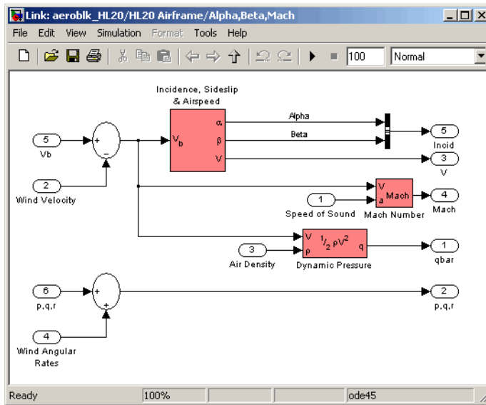
Additional Computed Parameters for HL-20 Airframe Model (Alpha, Beta, Mach Subsystem)
